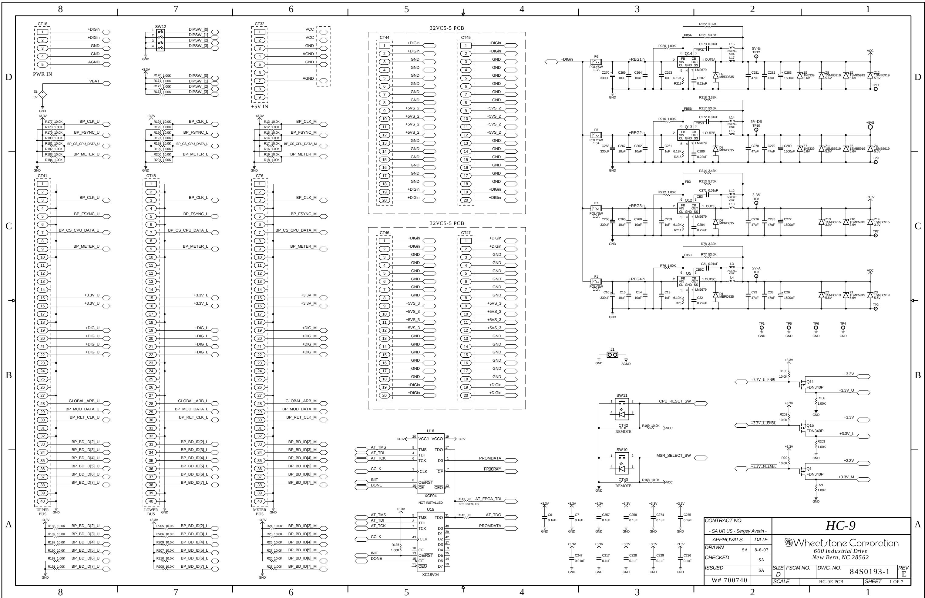
HC-9 Host Controller Card Schematic - Sheet 1 of 7
